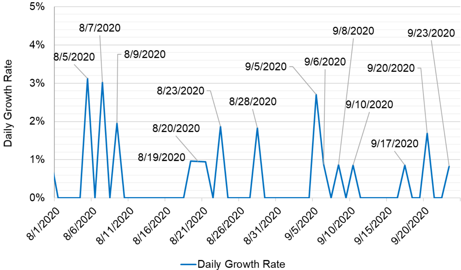
Daily Growth Rate - August 1, 2020 to Present
